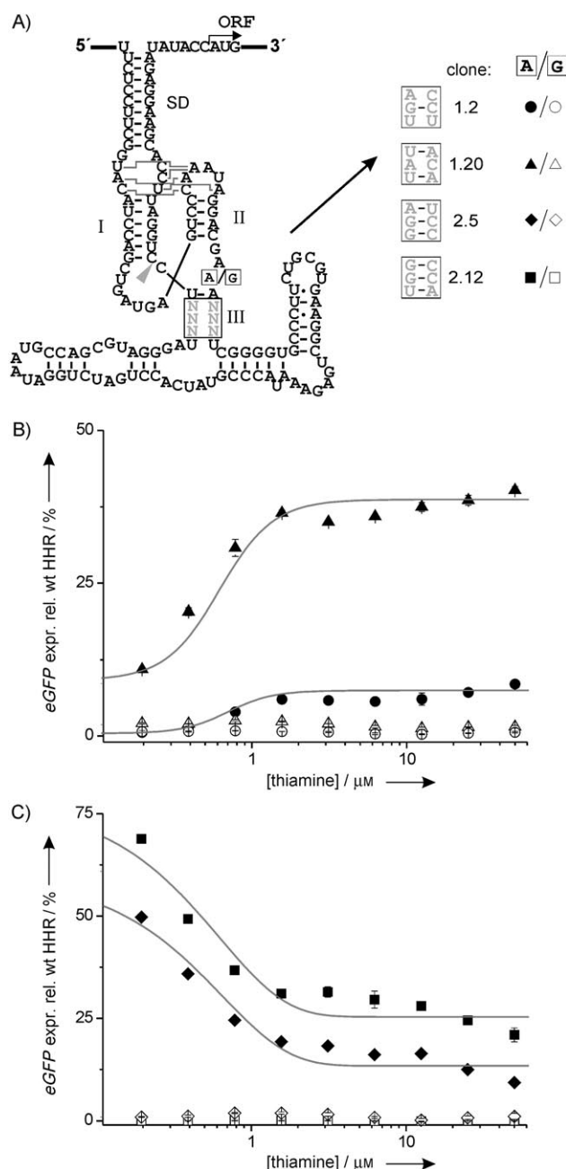
Figure 3. Characterization of individual clones: A) Sequences of two activating and two inhibiting switches: clones 1.2, 1.20, 2.5, and 2.12 (SD = Shine-Dalgarno sequence). B, C) Dependence of gene expression on thiamine concentration (y axis: eGFP expression relative to that with the wt HHR). Thiamine was added to the growth medium, and eGFP was detected in outgrown cultures. Closed symbols: clones as depicted in A, open symbols: clones as in A with a ribozyme-inactivating mutation in the catalytic core (A→G).
